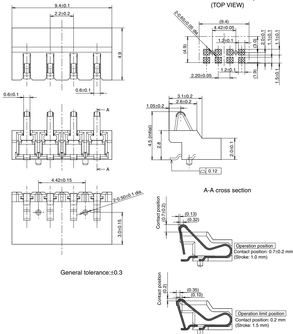
Recommended PC board pattern (TOP VIEW)
