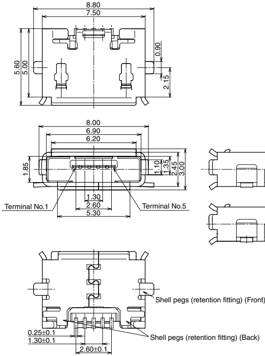
External dimensions
