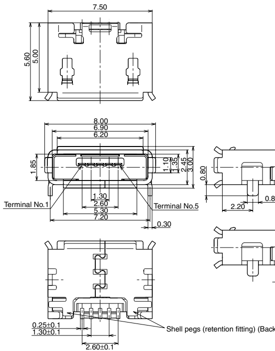
External dimensions
