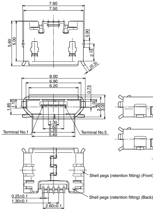
External dimensions
