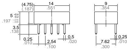
External dimensions Standard PC board terminal
