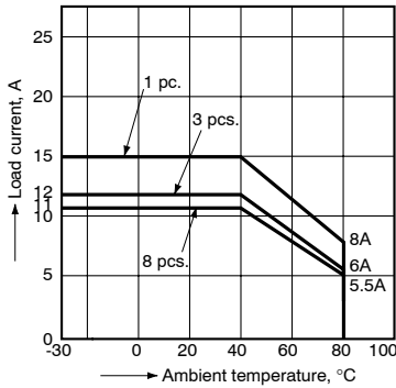
4-(1) Load current when contact mounted vs. ambient temperature characteristics Tested sample: AQK1211, AQK1231
