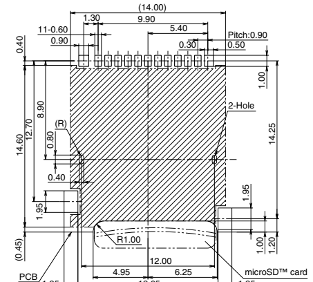
Recommended PC board pattern (TOP VIEW)
