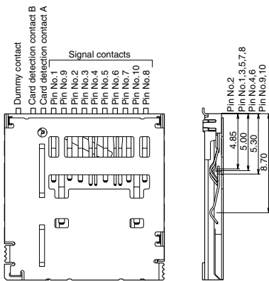
Pin arrangement
