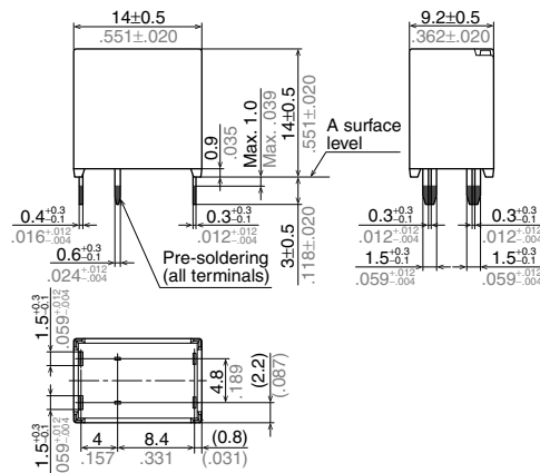
External dimensions
