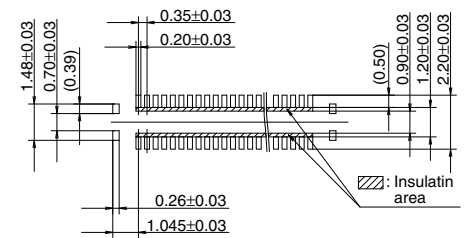
Recommended metal mask pattern Metal mask thickness: When 100μm (Signal terminal opening ratio: 70%) (Power terminal opening ratio: 77%)
