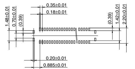
Recommended metal mask pattern Metal mask thickness: When 100μm (Signal terminal opening ratio: 70%) (Power terminal opening ratio: 77%)
