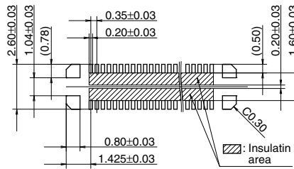
Recommended metal mask pattern Metal mask thickness: When 100μm (Signal terminal opening ratio: 70%) (Power terminal opening ratio: 100%)
